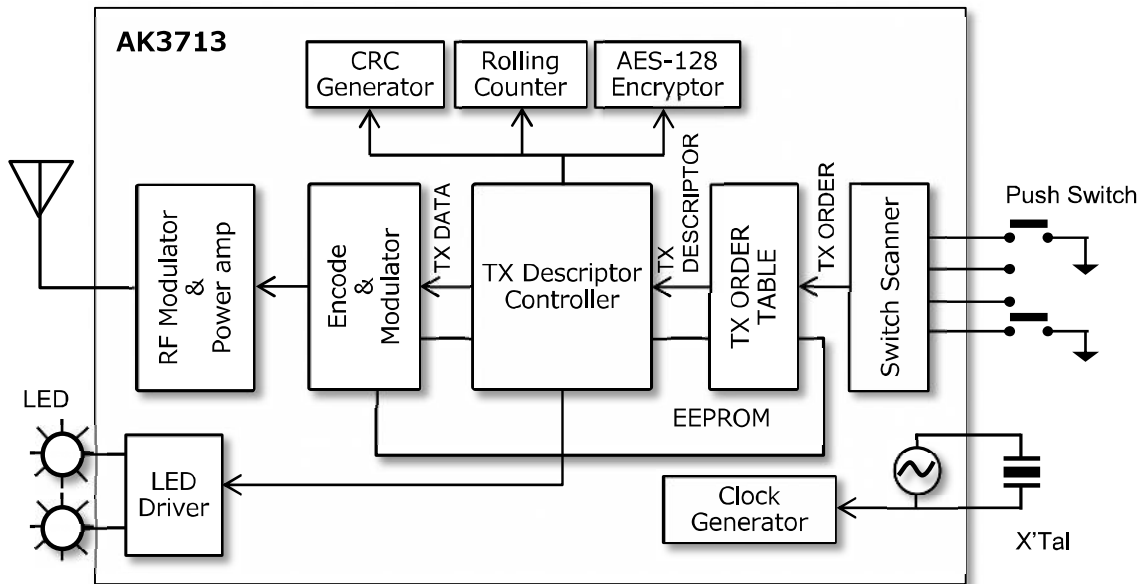
Figure 1 Block Diagram
