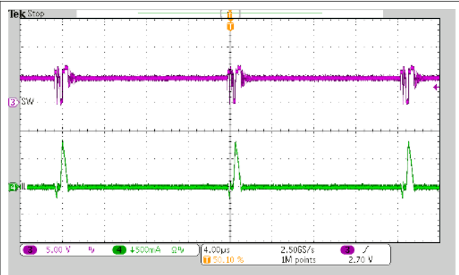
Figure 9-12. OTG Switching
