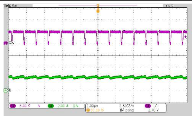
Figure 9-6. PFM Switching in Buck Mode
