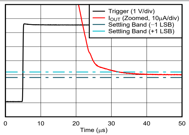
Figure 6-50. Current Output Setting Time, Falling Edge
