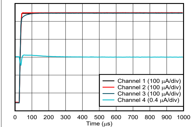
Figure 6-51. Current Output Power-On Glitch
