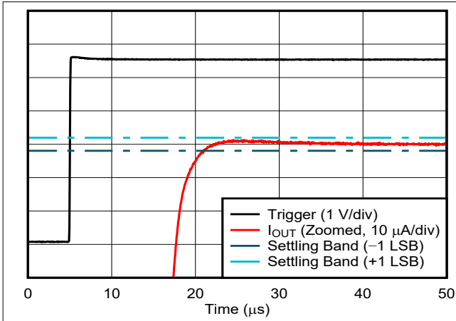
Figure 6-49. Current Output Setting Time, Rising Edge
