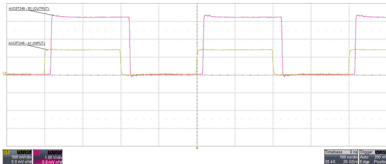
Figure 6. Translation Up (0.7 V to 3.3 V) at 2.5 MHz
