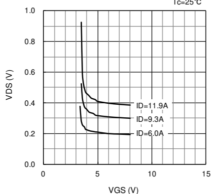
VDS-VGS characteristics (typical) Tc=25°C
