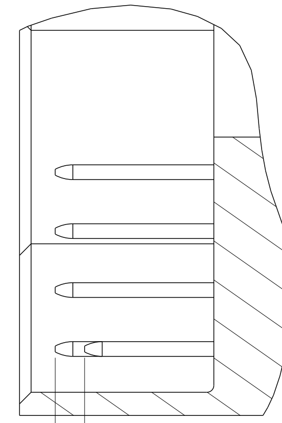
SECTION W-W SCALE 6:1 SIGNAL MATING SEQUENCE
