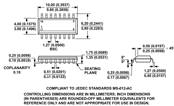
Figure 41. 16-Lead Standard Small Outline Package [SOIC_N] Narrow Body (R-16)
