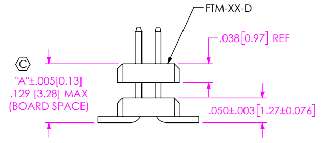
FIG 2 MW-10-03-X-D-120-073 SHOWN (DIFFERENT AS SHOWN, OTHERWISE SAME AS FIG 1)
