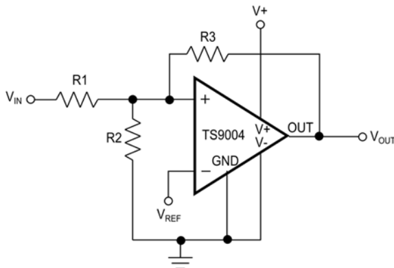
Figure 2. External Hysteresis
