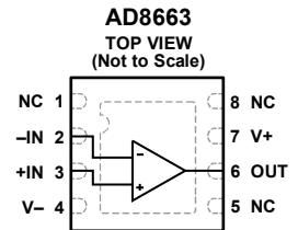
Figure 2. 8-Lead LFCSP (CP-8-13)
