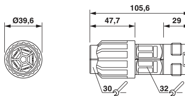
Dimensional drawing
