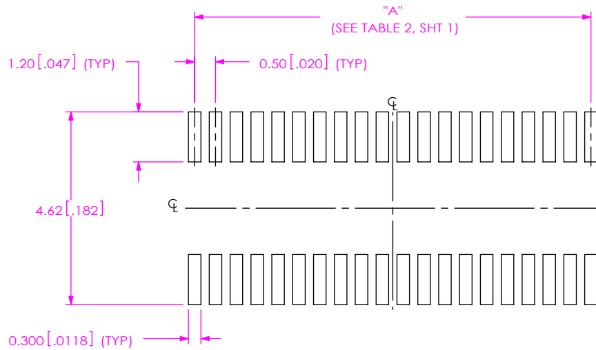
FIG 2 -20 POS SHOWN
