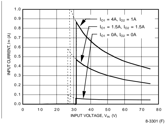
Figure 1. Typical HW025AF Input Characteristics at Room Temperature
