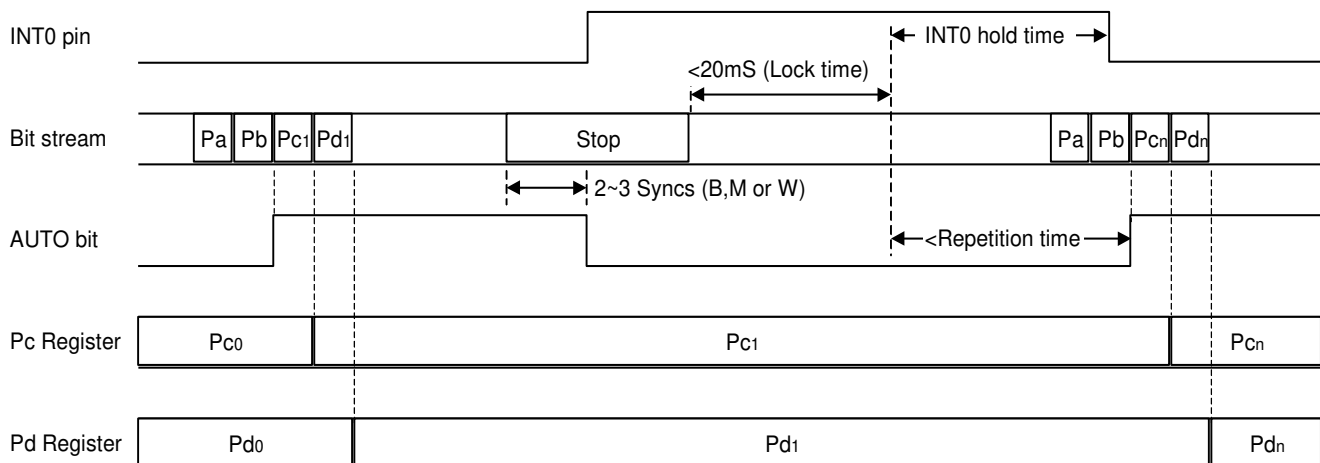
Figure 46. Timing Example 2
