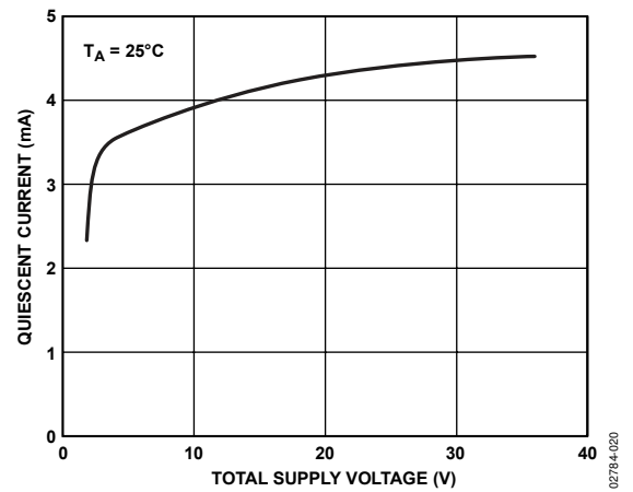
Figure 19. Quiescent Current vs. Total Supply Voltage
