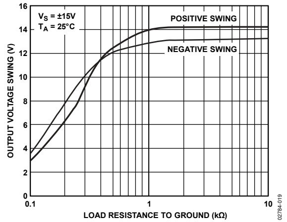
Figure 18. Output Voltage Swing vs. Load Resistance
