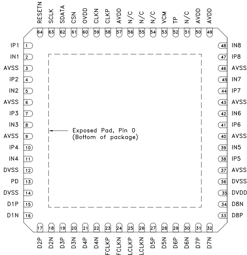
Figure 2. Package Diagram
