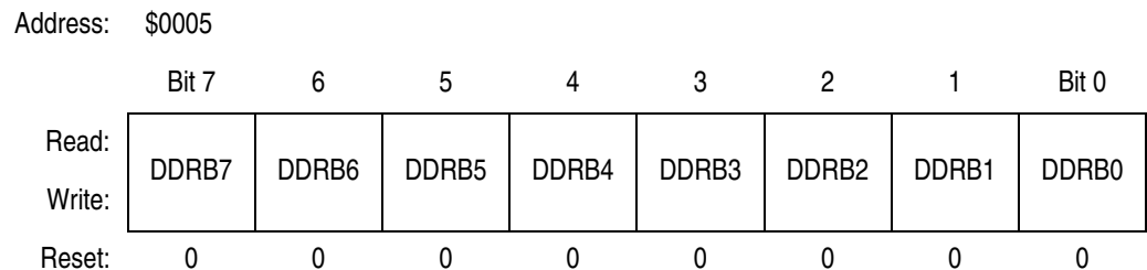
Figure 7-6. Data Direction Register B (DDRB)
