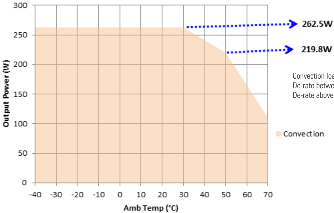
Derating Curve 15 V slotted cover
