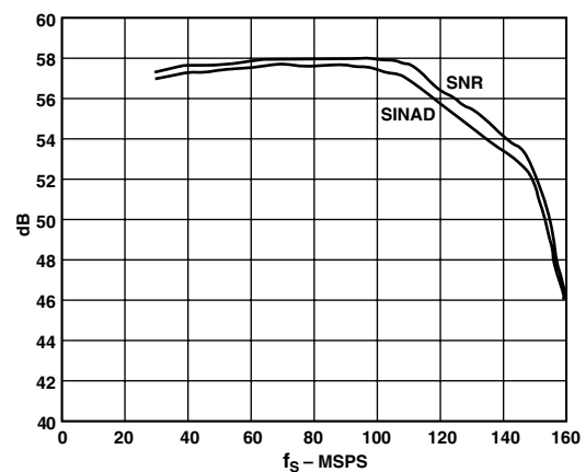
TPC 6. SNR vs. f_S ; f_{IN} = 10.3 MHz
