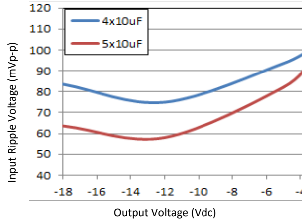
Figure 66. Input ripple voltage with 4x10 \mu F or 5x10 \mu F input ceramic capacitors (max load).
