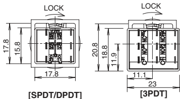
[SPDT/DPDT]
