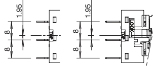
[3PDT]
