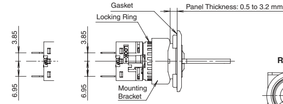
[SPDT/DPDT]
