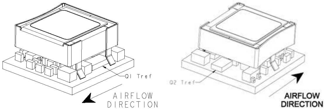
Figure 49. Preferred airflow direction and location of hot spot of the module (Tref).
