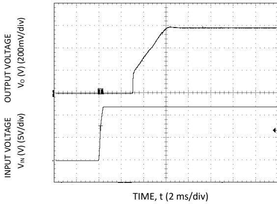
Figure 31. Start-up Using Input Voltage ( V_{IN} = 12V, I_o = I_{o,max} ), V_o = 0.6 V
