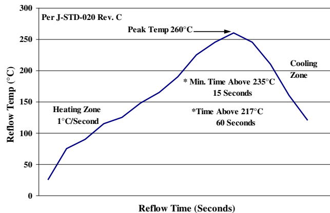
Figure 55. Recommended linear reflow profile using Sn/Ag/Cu solder.
