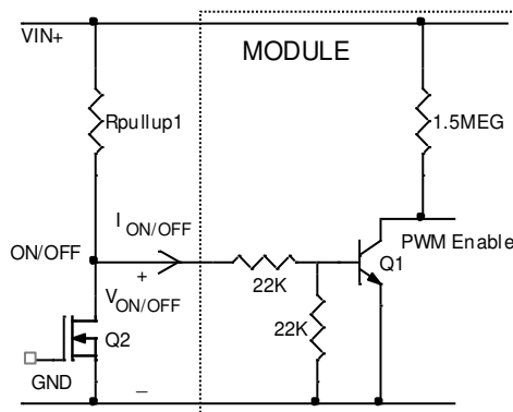
Figure 43. Circuit configuration for using negative On/Off logic
