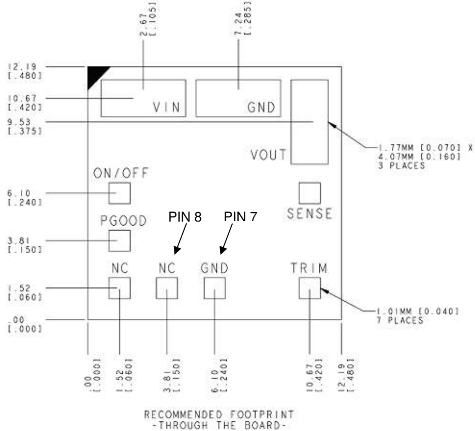
Figure 53. Recommended pad layout
