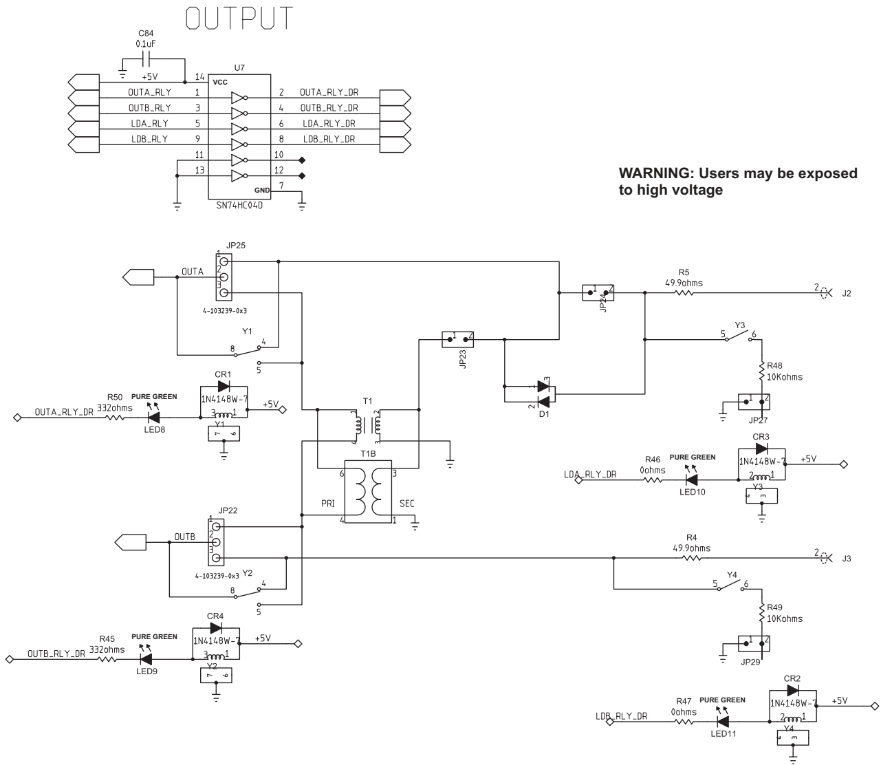
Figure 16. Schematic (3 of 8)
