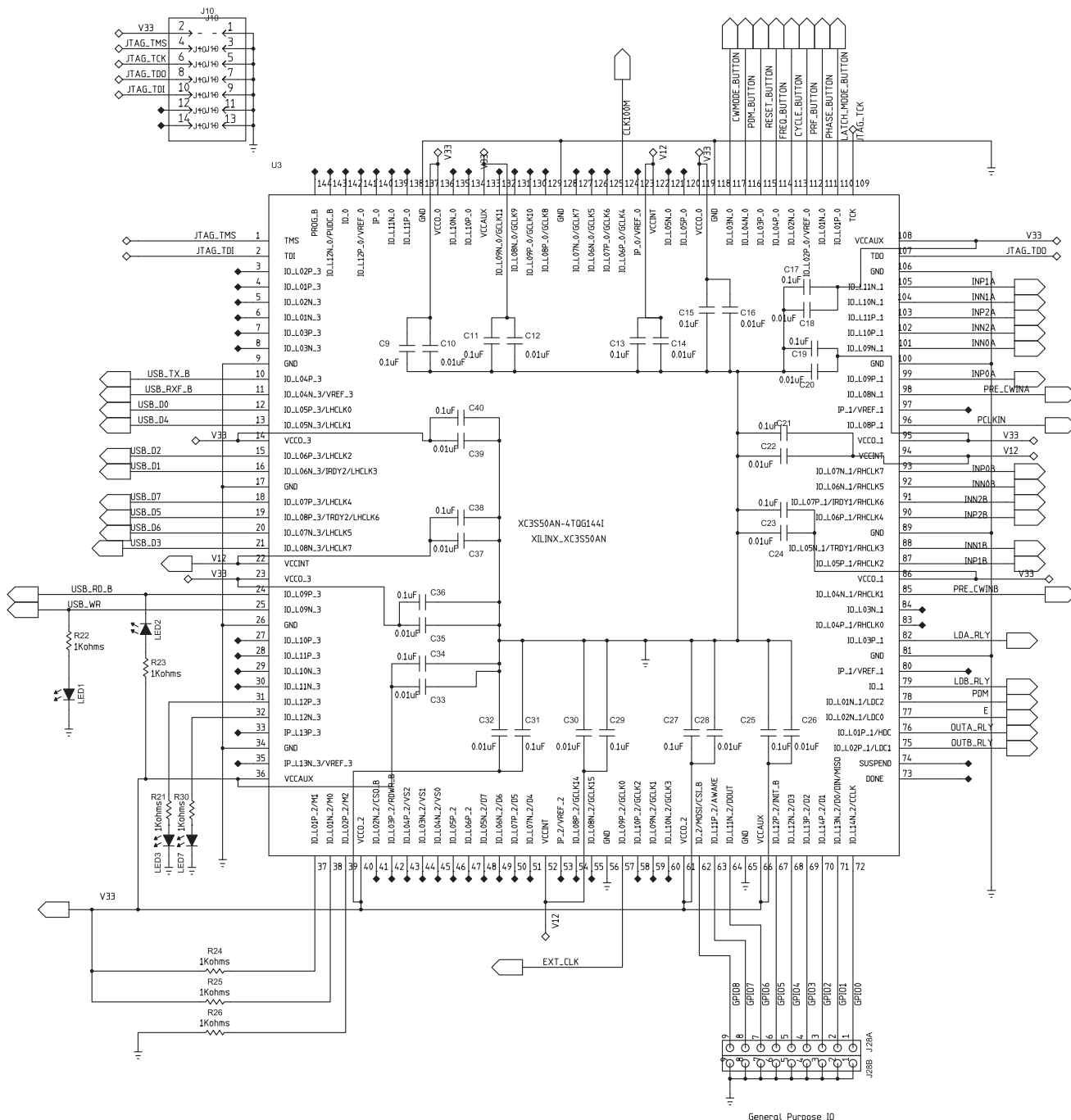
Figure 20. Schematic (7 of 8)
