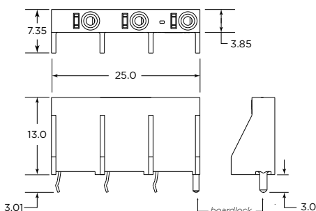
3 position in-line screwless wire connector
