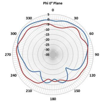
1990 MHz Radiation Pattern
