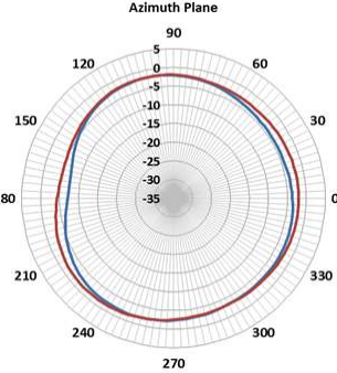
1850 MHz Radiation Pattern
