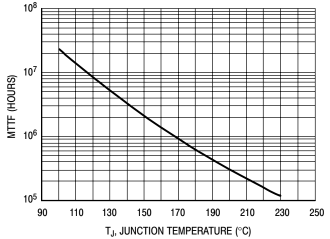
Figure 12. MTTF versus Junction Temperature This above graph displays calculated MTTF in hours when the device is operated at V_{DD} = 28 Vdc, P_{out} = 58 W Avg., and \eta_D = 34\% . MTTF calculator available at http://www.freescale.com/rf . Select Tools (Software & Tools)/Calculators to access MTTF calculators by product.
