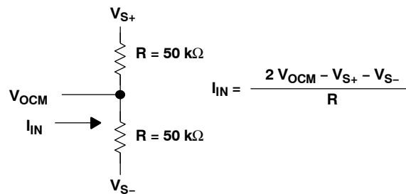
Equivalent Input Circuit for V_{OCM} Figure 102
