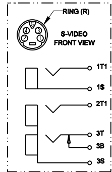
SCHMATIC
