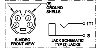
SCHMATIC
