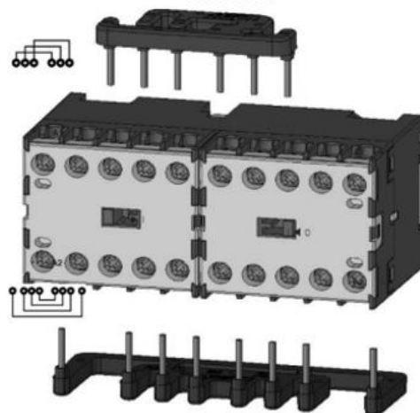
Reversing Starter Connector K0W-VB for reversing contactors K0W05D...
