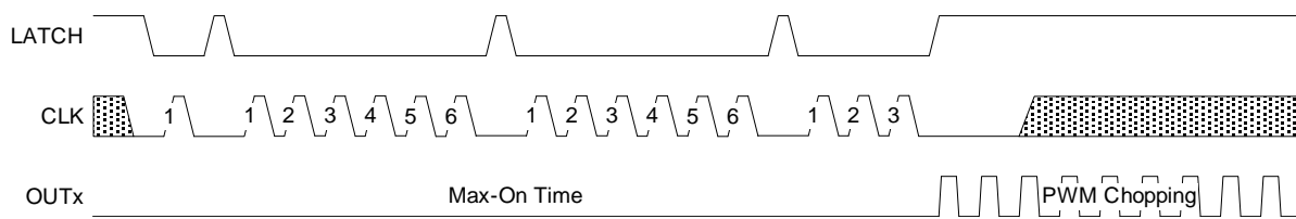
Figure 28. PWM Start Command
