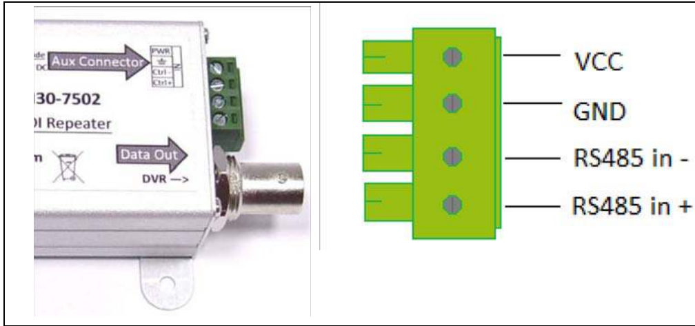
FIGURE 1-5: DVR SIDE
