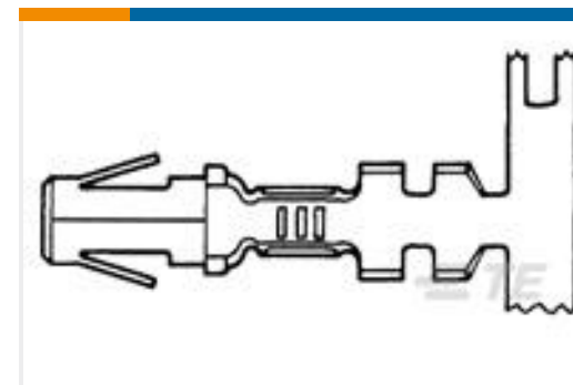
TE Part #61626-2 .140 DIA SOK 20-14 PTPPHBZ
