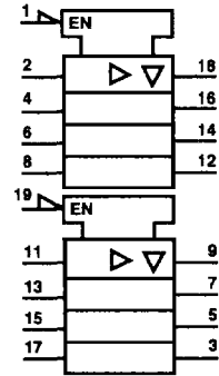
CD74FCT244, CD74FCT244AT
