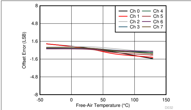
Figure 6-36. Offset Error vs Free-Air Temperature ( \pm 10\text{ V} , Across Channels)
