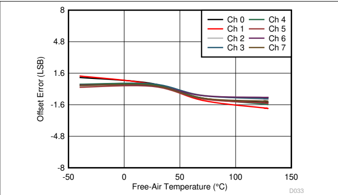
Figure 6-37. Offset Error vs Free-Air Temperature ( \pm 5\text{ V} , Across Channels)
