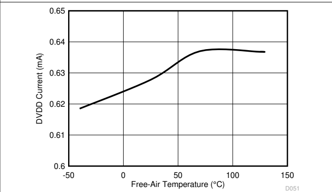
Figure 6-41. DVDD Current vs Free-Air Temperature
