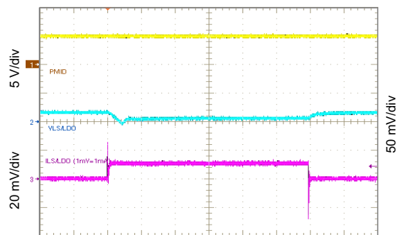
V_{LSLDO} = 1.2 \text{ V} Figure 10-48. 1.2 V_{LSLDO} Load Transient, 0 to 10 mA
