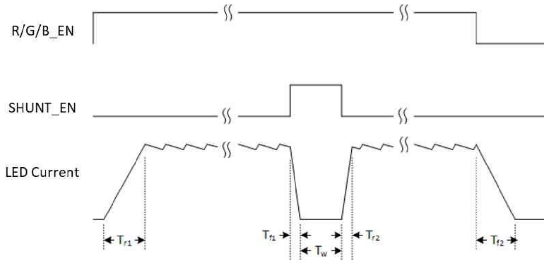
Figure 2-6. LED Driver Timing Specifications
