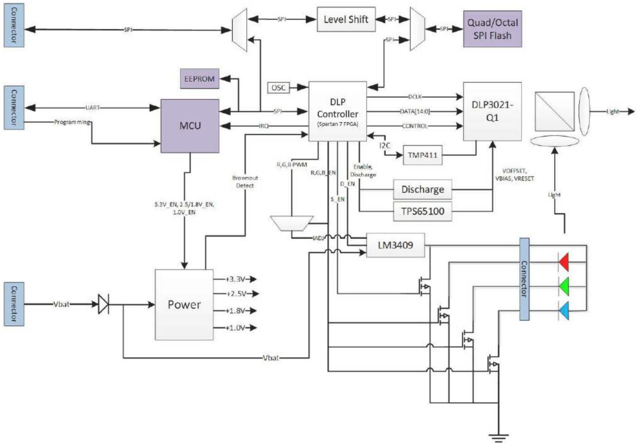
Figure 2-1. DLP3021LEQ1EVM Block Diagram
