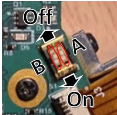
Figure 2-3. Operating Mode Switches: Electronics Board S1-A and S1-B Switches
