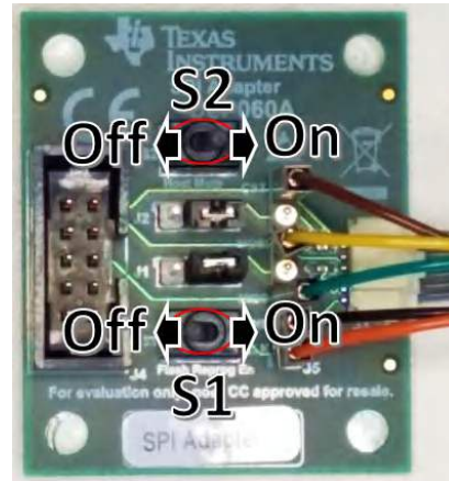
Figure 2-4. Operating Mode Switches: SPI Adapter Board S1 and S2 Switches
