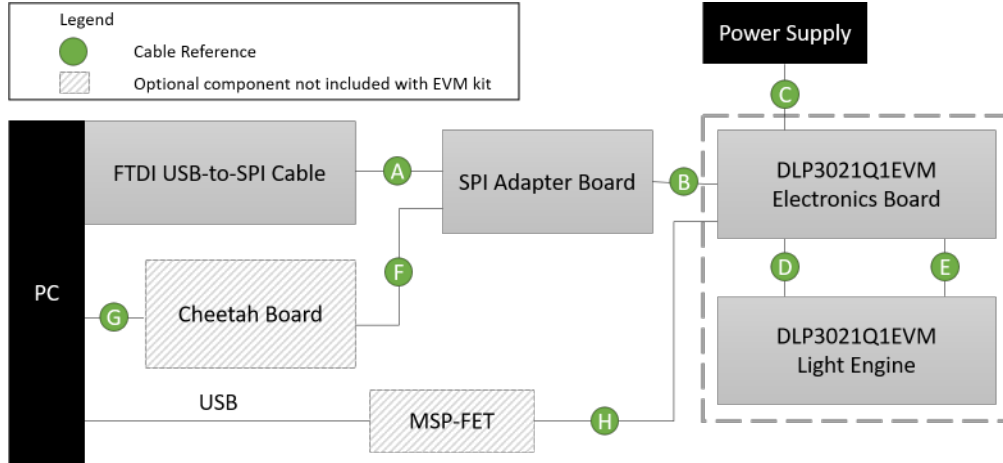
Figure 3-1. Cable Connections
