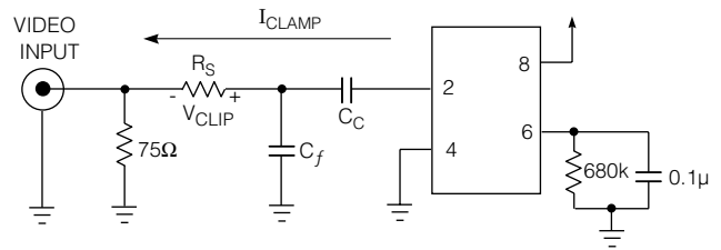
Fig. 22 Simple Chrominance Filtering
