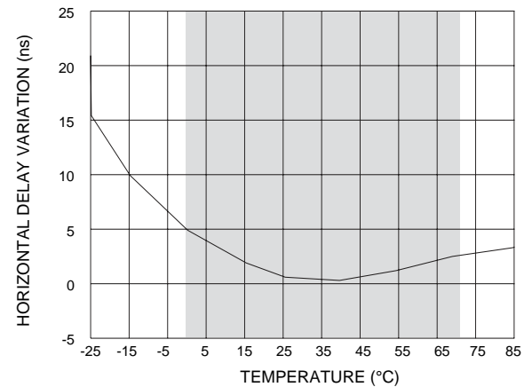
Fig. 11 Horizontal Delay Variation vs Temperature
