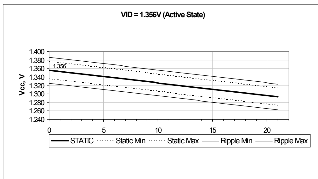
Figure 2. Illustration of Active State V_{CC} Static and Ripple Tolerances
