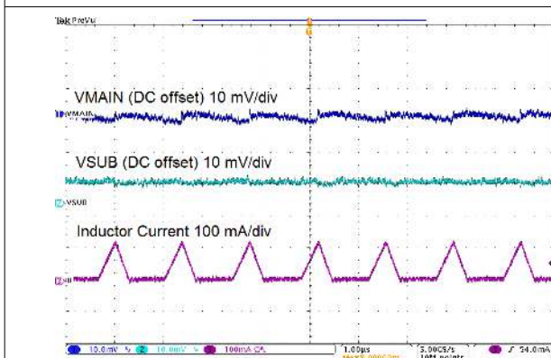
TPS610981 I_{(MAIN)} = 0 \text{ mA} I_{(SUB)} = 10 \text{ mA} MODE = H V_{IN} = 1.5 \text{ V}
