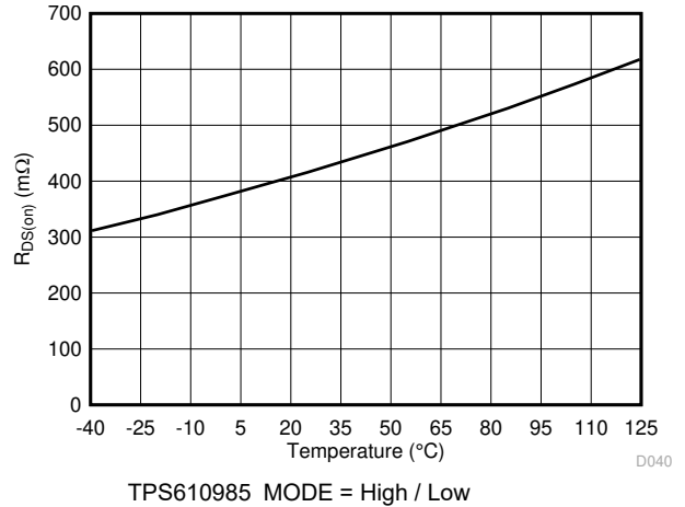
Figure 7-14. Low Side Switch On Resistance vs Temperature
