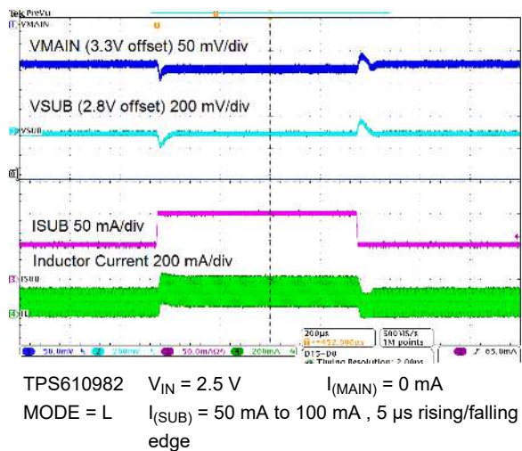
Figure 9-34. LDO Load Transient Response
