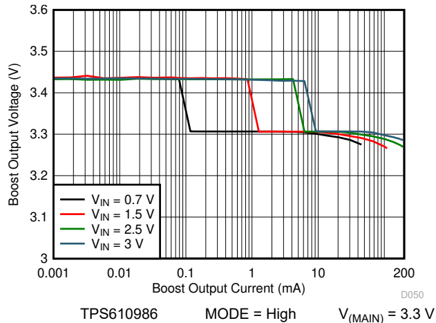
Figure 7-37. Boost Load Regulation (Active Mode)
