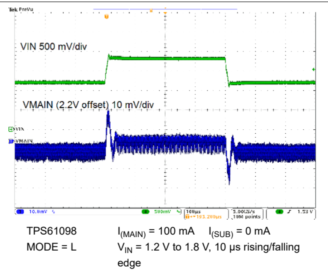
Figure 9-27. Line Transient Response
