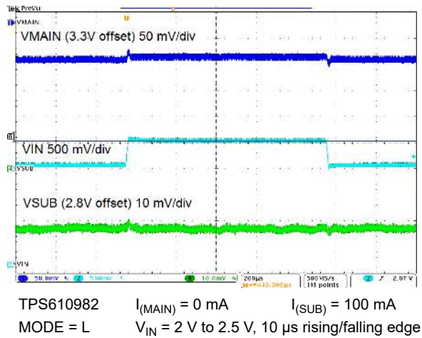
Figure 9-32. Line Transient Response
