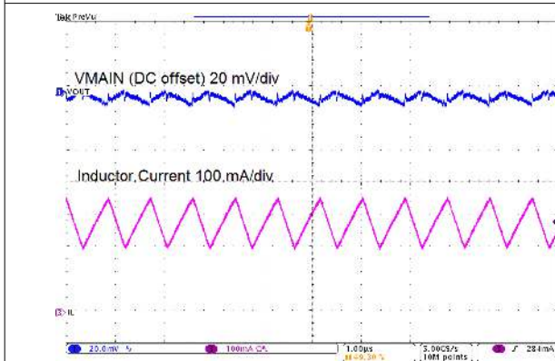
TPS610981 I_{(MAIN)} = 100 \text{ mA} I_{(SUB)} = 0 \text{ mA} MODE = L V_{IN} = 1.5 \text{ V}
