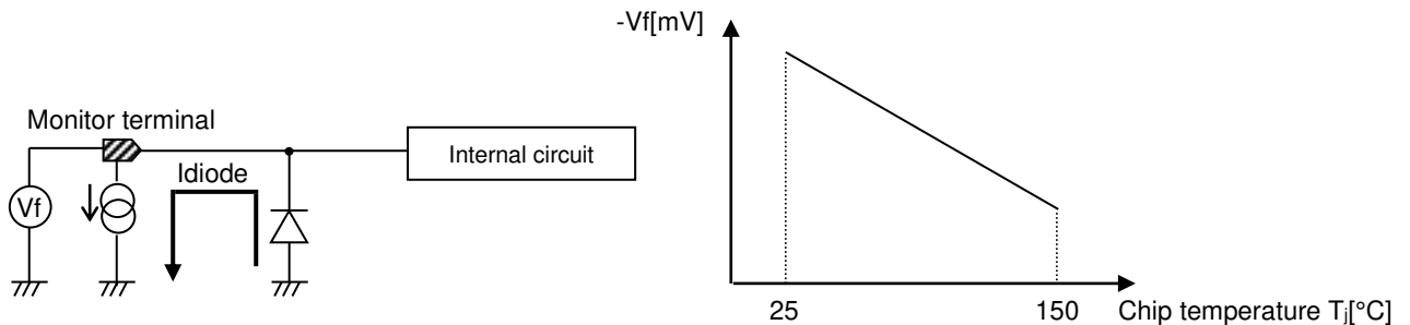
Figure 9. Model diagram for measuring chip temperature
