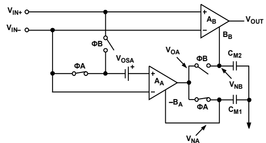
Figure 50. Auto-Zero Phase of the AD8551/AD8552/AD8554
