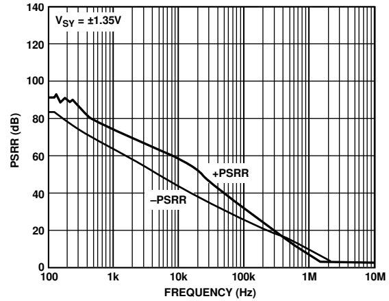
Figure 34. PSRR vs. Frequency at ±1.35 V
