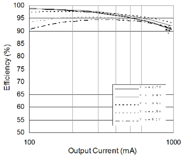
Figure 5. AS1346 Efficiency vs. V_{IN} , V_{OUT1} = 3.3V
