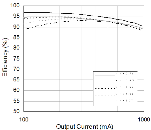
Figure 7. Efficiency vs. I_{OUT} , V_{OUT1} = 2.5V
