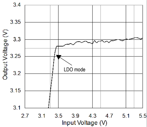
Figure 11. AS1346 Line Regulation, V_{OUT1} = 3.3V
