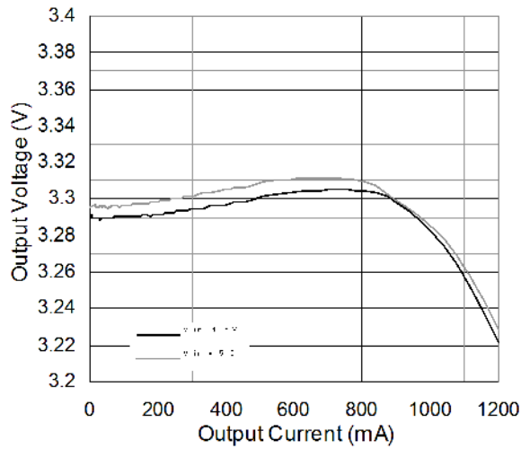
Figure 9. AS1346 Load Regulation; V_{IN} = 4.0V , V_{OUT1} = 3.3V
