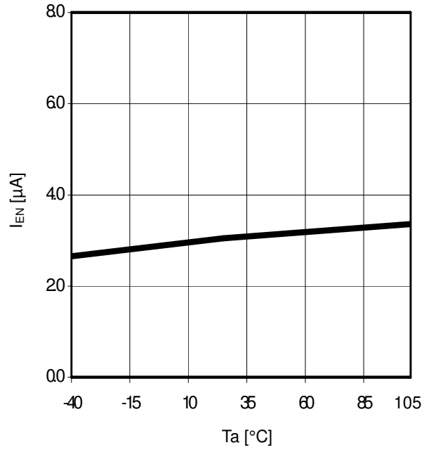
Figure 24. T_a - I_{EN}
