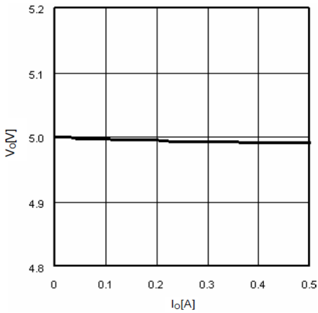
Figure 25. I_O - V_O
