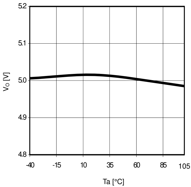
Figure 21. Ta-V_O ( I_O=0mA )
