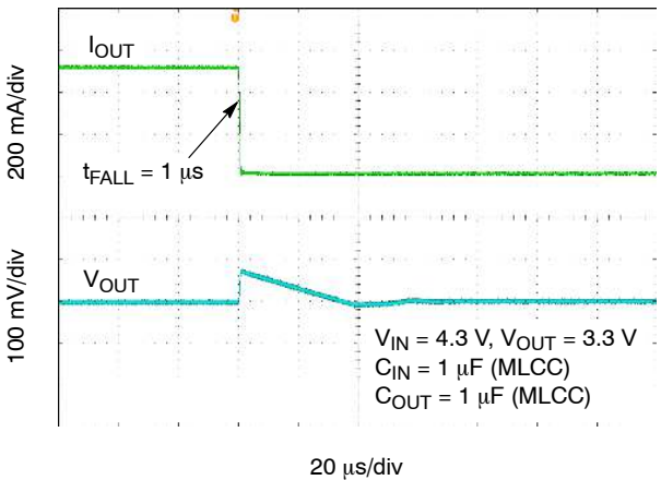
Figure 35. Load Transient Response – 450\text{ mA to }1\text{ mA} - V_{OUT} = 3.3\text{ V}
