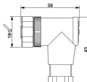
Dimensioned drawing
