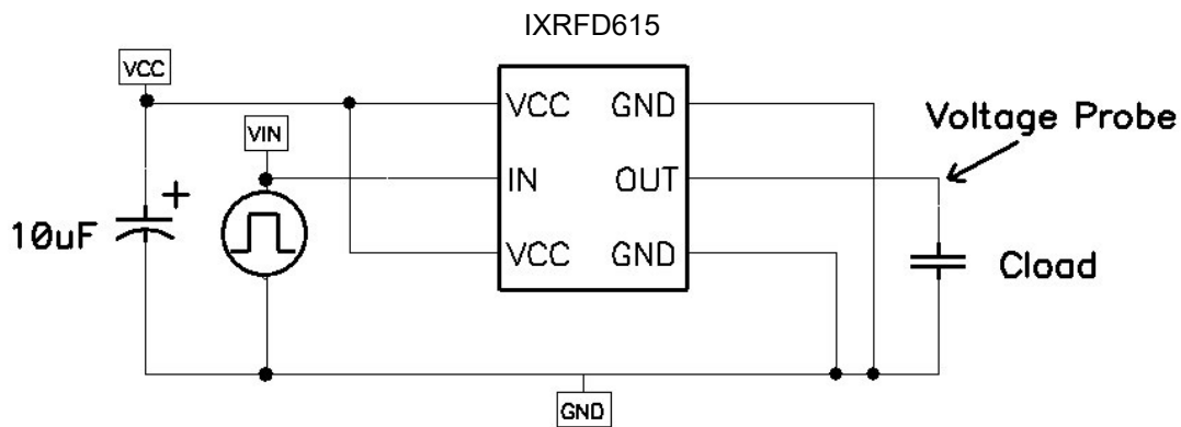
Fig. 21 Test Circuit Diagram
