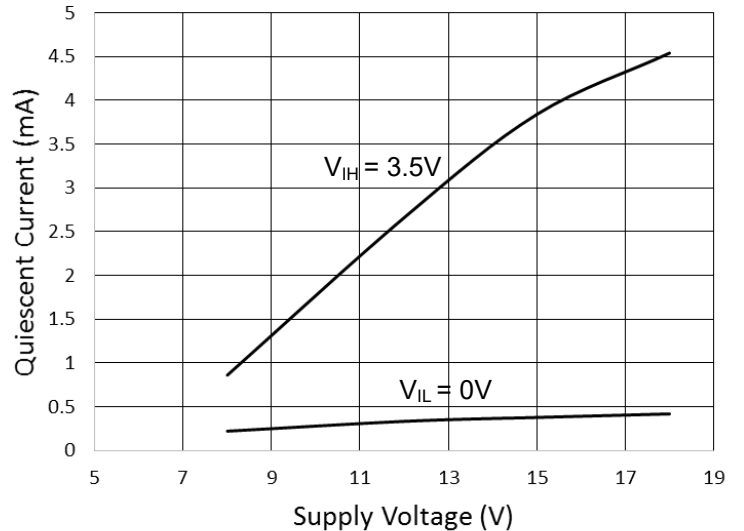
Fig. 7 Quiescent Current vs. Supply Voltage
