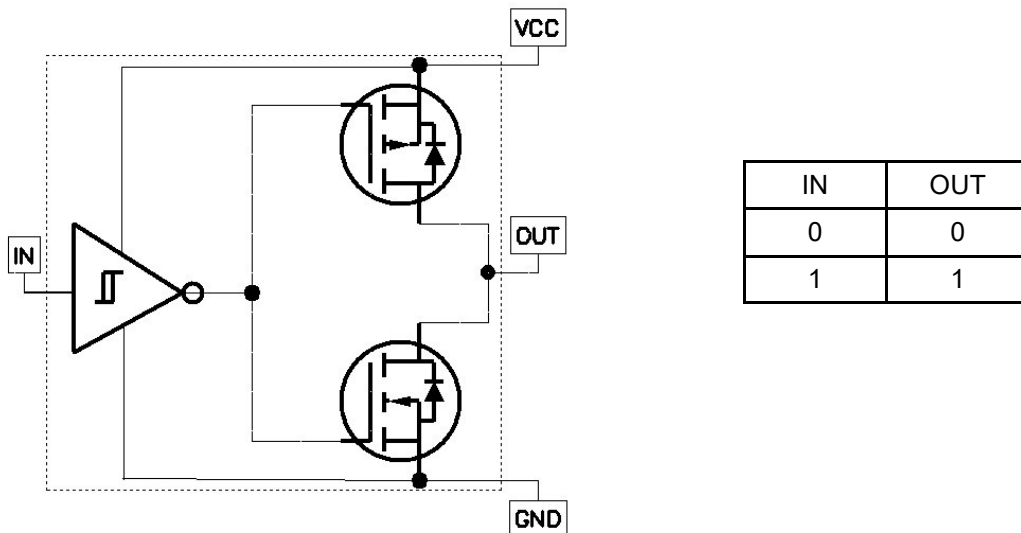
Fig. 1- Block Diagram and Truth Table
