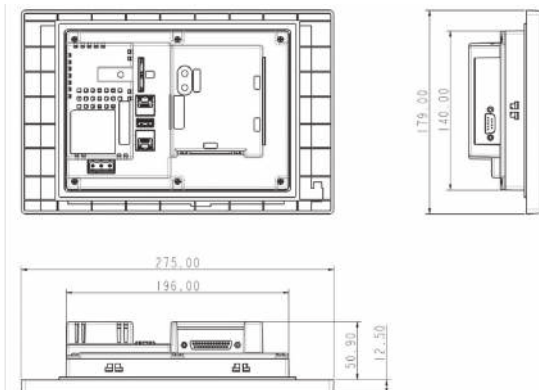
Dimensional drawings of the 10" HMI
