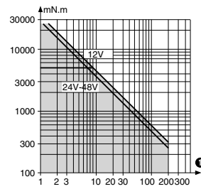
Nominal speed and torque curves 80 817 0
