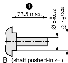
Gearbox shaft 79 290 064
