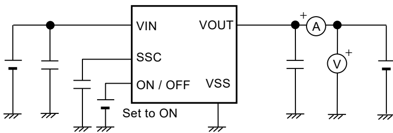
Figure 5 Test Circuit 3
