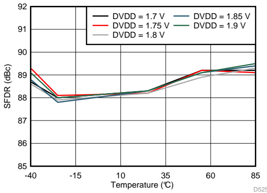
Figure 56. Spurious-Free Dynamic Range vs DVDD Supply and Temperature (30 MHz)
